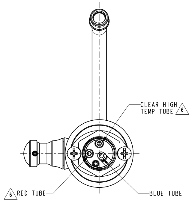
BOTTOM VIEW SCALE .500
