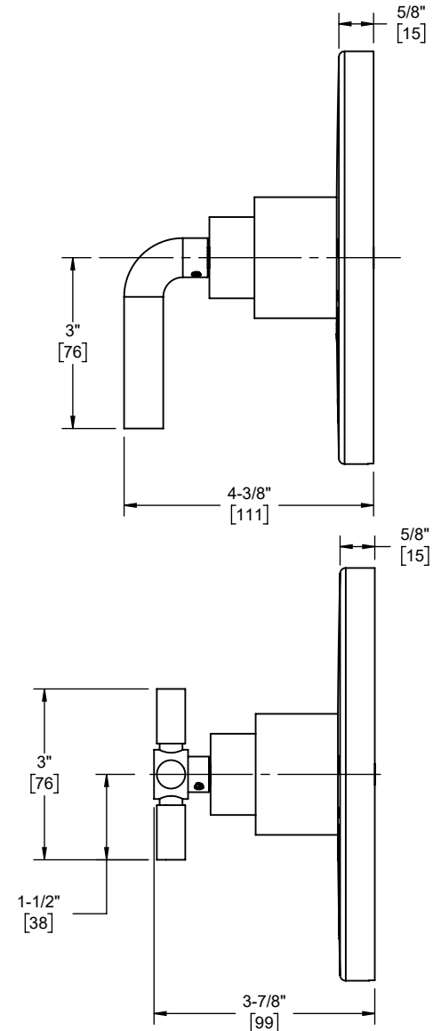
(TO-PB2L-30X SHOWN)
