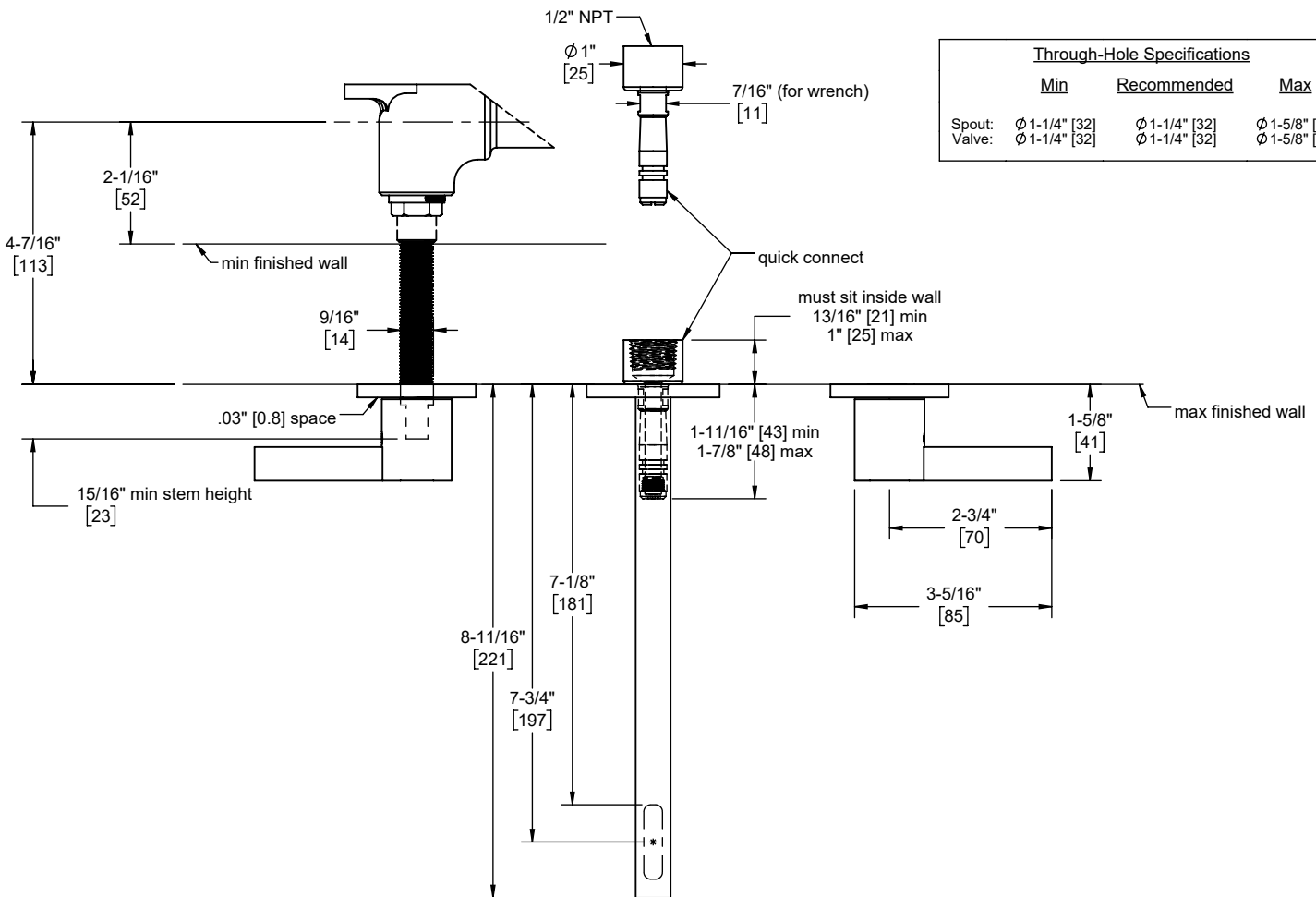
TO-VE302-7 shown
