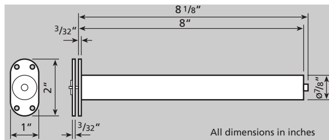
Perko® R21 Round Plates (extended version)
