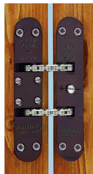
Perkomatic® R85.BMA
