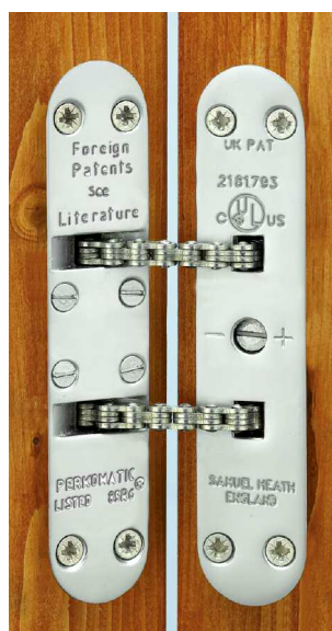
Perkomatic® R85.SCP
