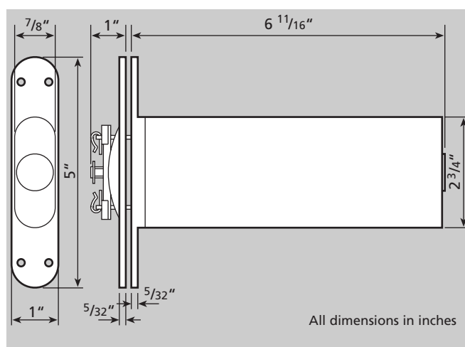
Perkomatic® R85
