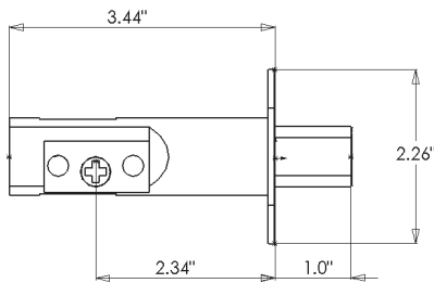
2-3/8" Deadbolt
