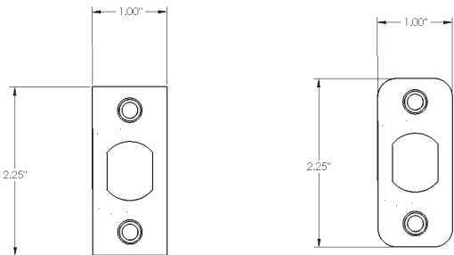
Square Deadbolt
