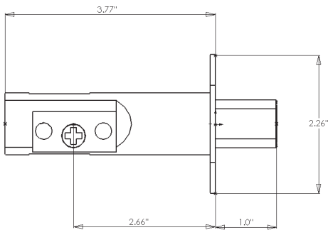
2-3/4" Deadbolt
