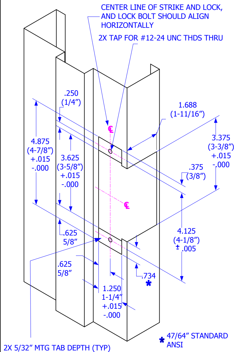
FIG. 4 FRAME PREPARATION – 2930 Electric Strike
