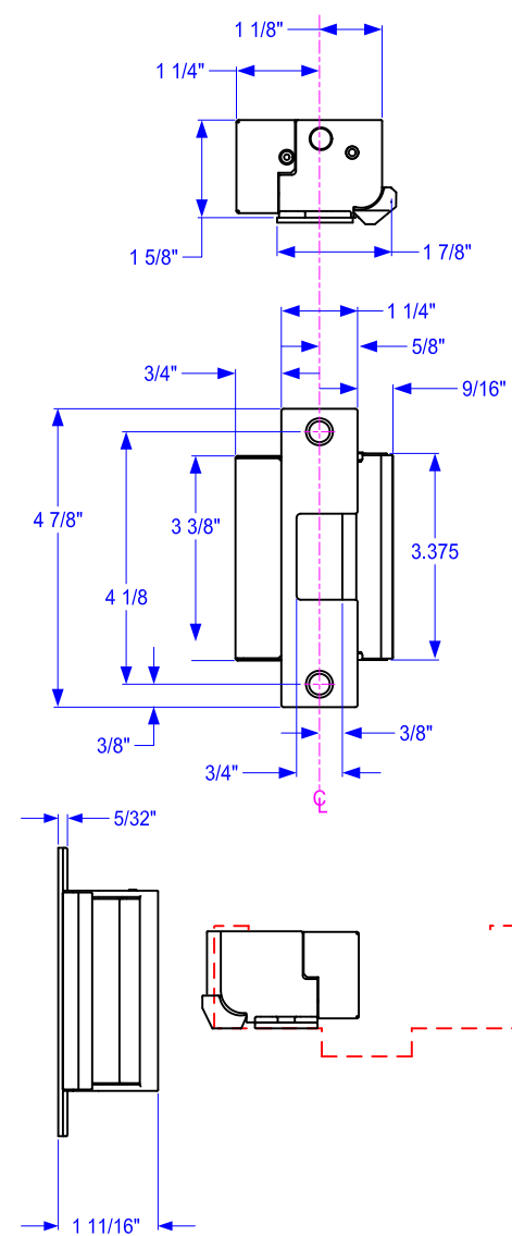
FIG. 5 STRIKE DIMENSIONS
