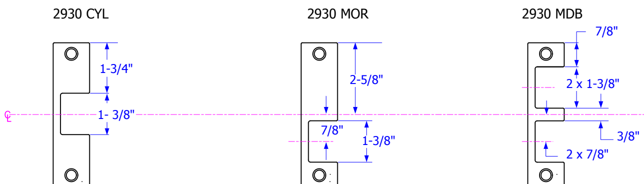
FIG. 6 FACE PLATES – All faceplates are interchangeable for application requirements
