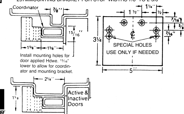
297M MOUNTING BRACKET FOR STOP WIDTHS 7/8" TO 2-3/8"
