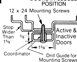
297M MOUNTING BRACKET FOR STOP WIDTHS 7/8" TO 2-3/8"
