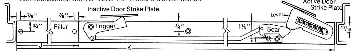
297D COORDINATOR WITH 297F FILLER PLATE. DOORS IN OPEN POSITION
