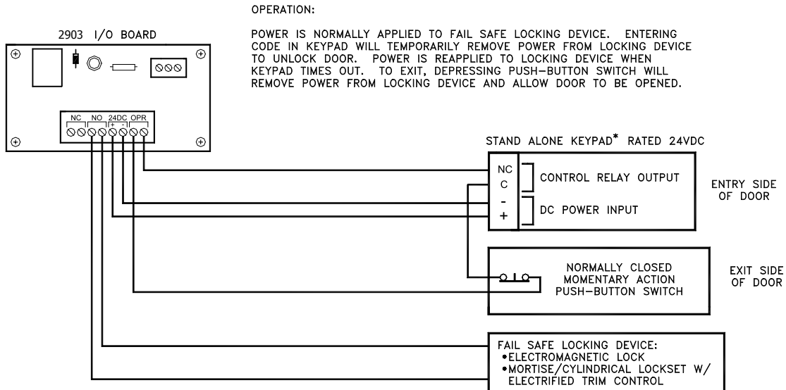
Figure 1 Wire scheme for a typical fail safe system
