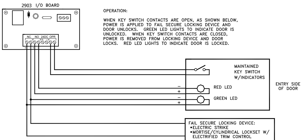
Figure 2 Wire scheme for a typical fail secure system
