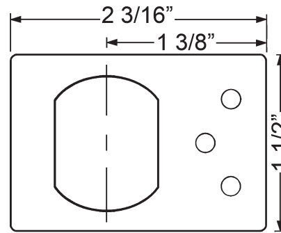
Stabilizer Plate
