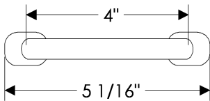
CK318 Sash Cabinet Pull, 4"
