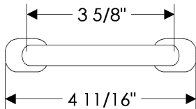
CK310 Sash Cabinet Pull, 3 5/8"
