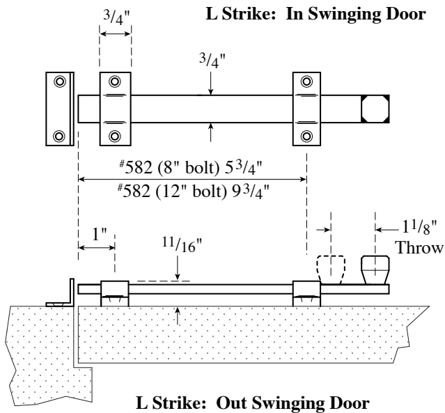
Single Lock Bracket for Pad Lock (Bolt Shown in Unlocked Position)
